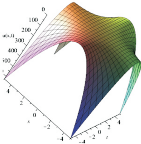
Figure 6a: 3D plot of example 5 at x = -5..5 , t = -5..5
