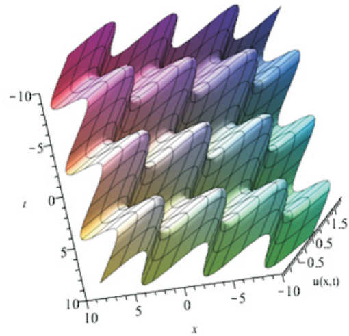
Figure 3a: 3D plot of example 3 at x=-10..10 , t=-10..10
