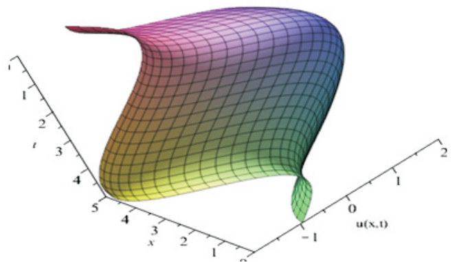
Figure 3b: 3D plot of example 3 at x=0..5 , t=0..5
