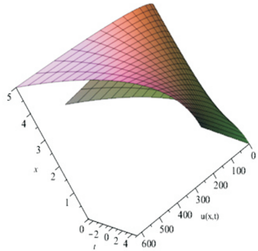
Figure 6b: 3D plot of example 5 at x = 0..5 , t = -5..5
