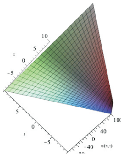
Figure 5a: 3D plot of example 5 at x = -10..10 , t = -10..10
