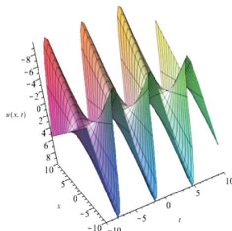
Figure a: plot of example 1 at x = -10..10 , t = -10..10
