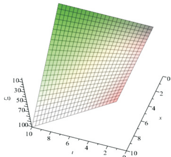
Figure 5b: 3D plot of example 5 at x = 0..10 , t = 0..10
