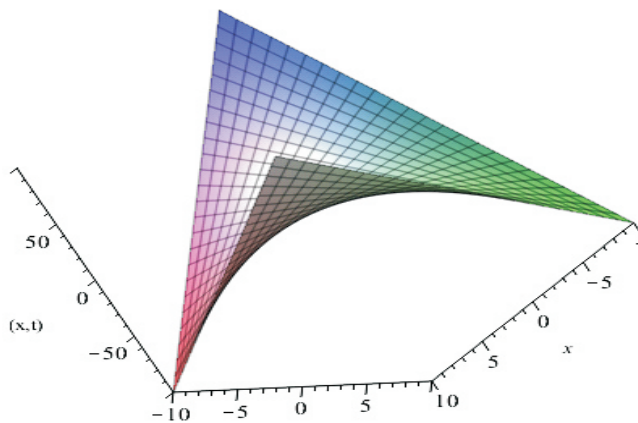
Figure 4b: 3D plot of example 4 at x = -10..10 , t = -10..1
